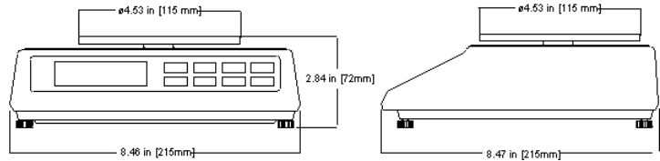
PBS-300 & PBS-600
