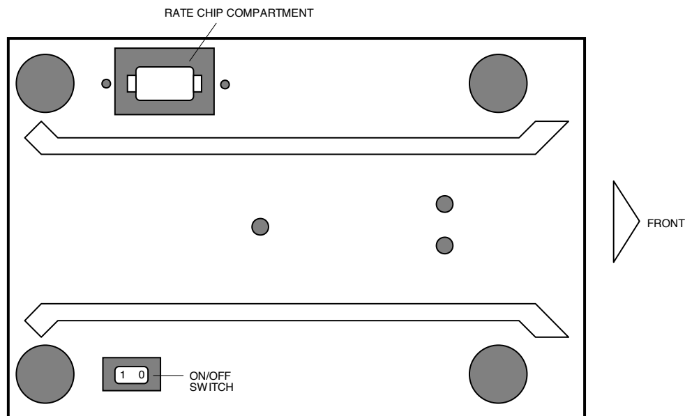
Underside of SPS-30 – Rate chip compartment cover is removed
