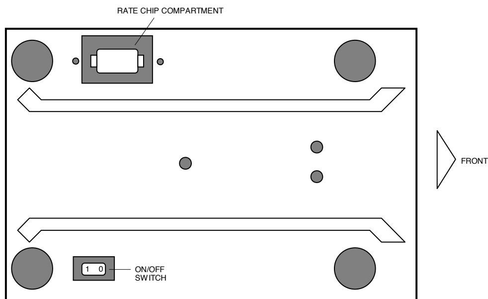
Underside of SPS-30 Plus – Rate chip compartment cover is removed
